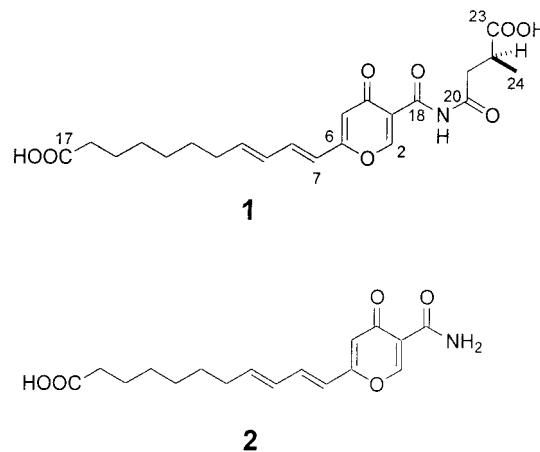
Scheme 1. Structures of Microsphaerones A ( 1 ) and B ( 2 )
